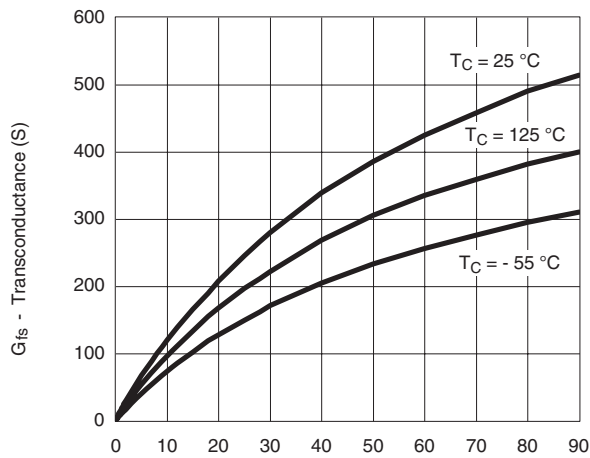
Transconductance
